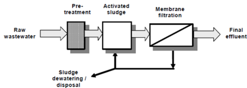
Figure 2: Conceptual diagram of a Membrane Bioreactor System [3].
