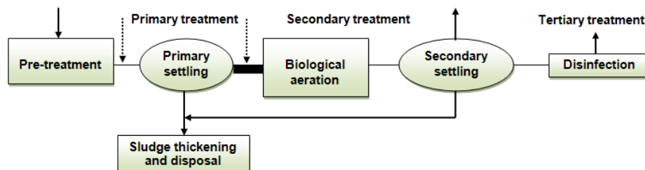
Figure 1: Conceptual diagram of a typical activated sludge process
