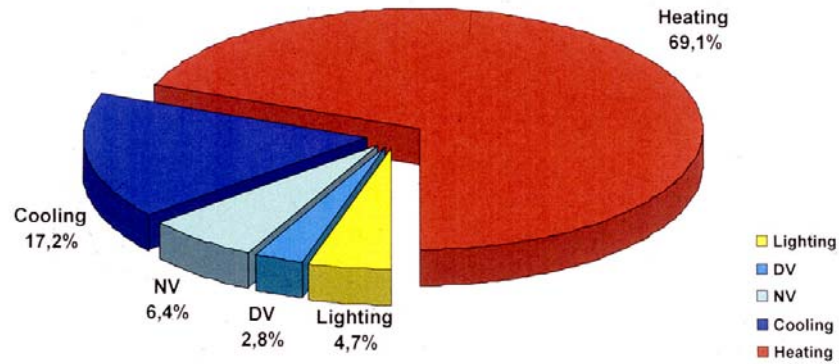
PERCENTAGE OF ANNUAL ENERGY CONSUMPTION 1998
