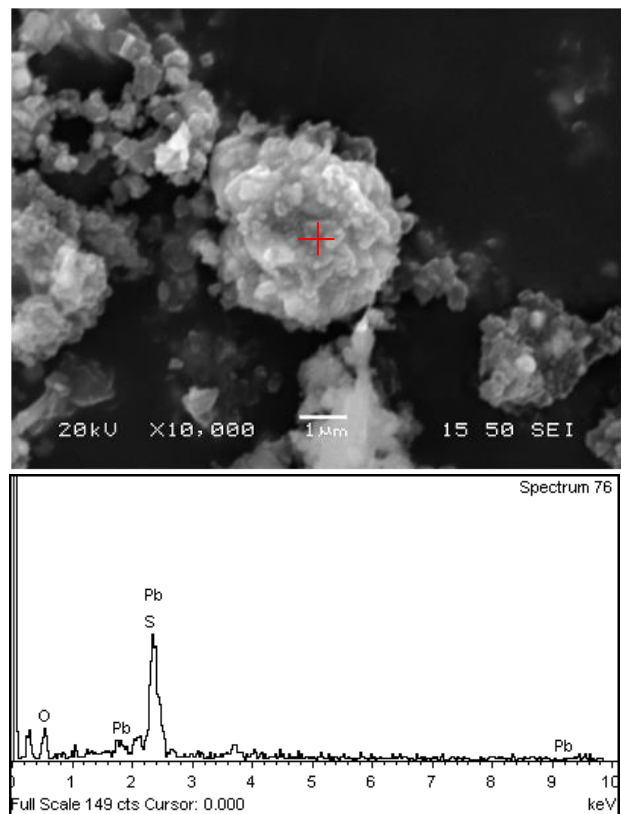
Figure 19: SEM image of the 4 th step leach residue (95°C, 3N H 2 SO 4 , 20% pulp density, 120 min). An aggregate of lead sulphate crystallites.
