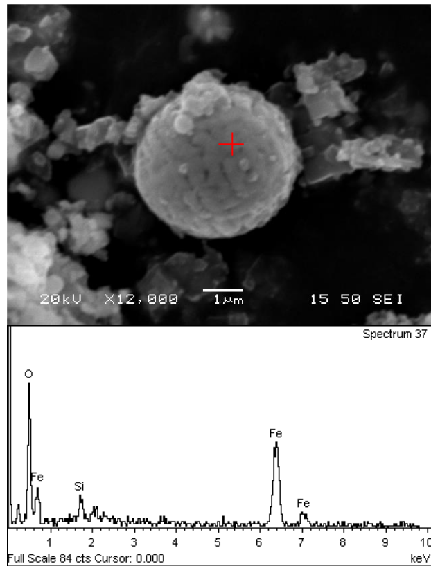
Figure 16: SEM image of the 3 rd step leach residue (95°C, 3N H 2 SO 4 , 20% pulp density, 120 min). A corroded by the acid spherical grain of magnetite.
