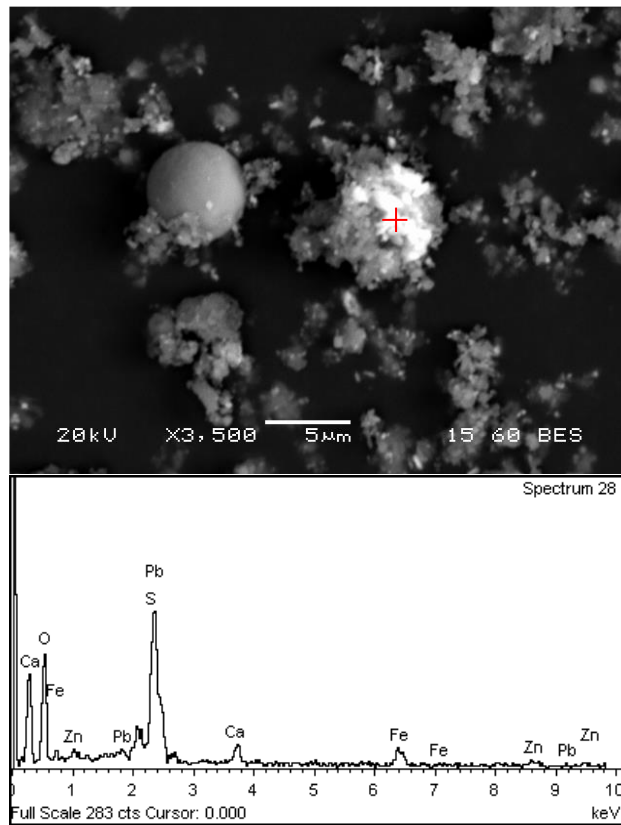
Figure 14: SEM image of the 3 rd step residue (95°C, 3N H 2 SO 4 , 20% pulp density, 120 min). A white crystal of lead sulphate.
