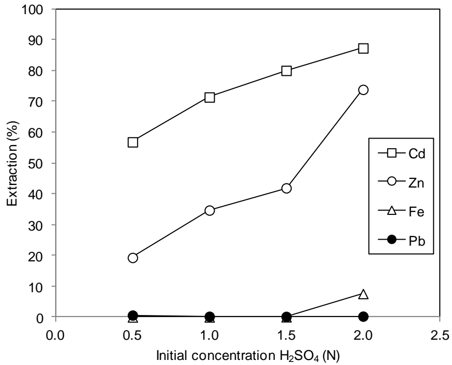
Figure 8: 2 nd step leaching. Extraction (%) of metals vs initial sulphuric acid concentration (25°C, 20% pulp density, 20 min).
