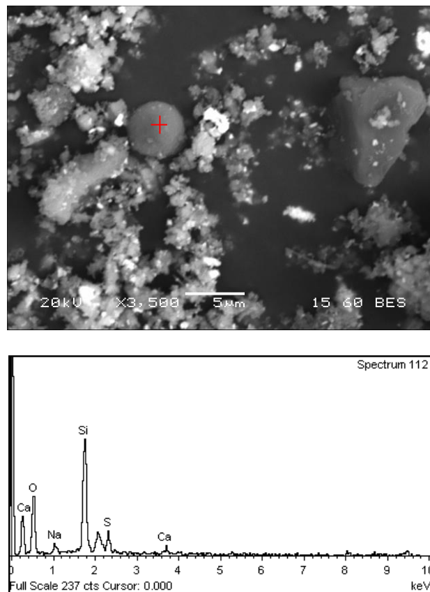
Figure 21: SEM images of the 4 th step leach residue (95°C, 3N H 2 SO 4 , 20% pulp density, 120 min). A silica grain.
