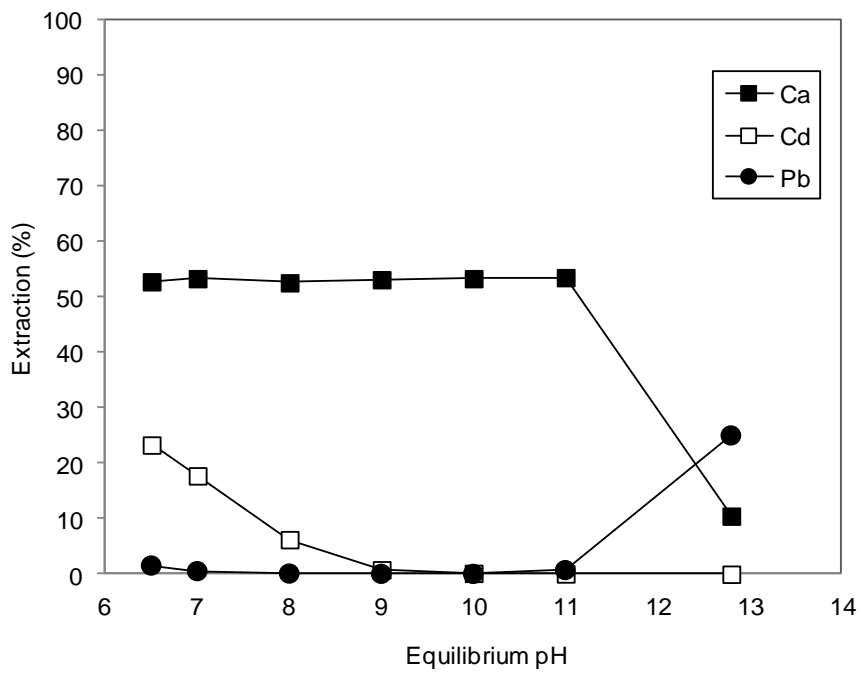
Figure 3: Water –washing of the EAF dust. Extraction (%) of metals vs equilibrium pH. (25°C, 20% pulp density, 60 min).
