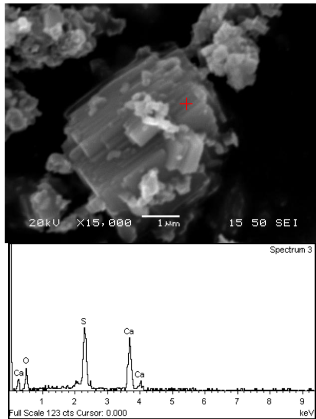
Figure 20: SEM image of the 4 th step leach residue (95°C, 3N H 2 SO 4 , 20% pulp density, 120 min). A calcium sulphate crystal.
