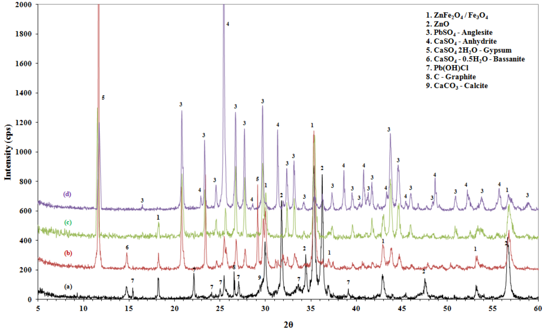
Figure 5: Mineralogical phases of leach residues produced at successive leach steps: (a) water-washed EAF dust (1 st step) (b) 25°C leach residue (2 nd step) (c) 95°C leach residue (3 rd step) (d) 95°C leach residue (4 th step).
