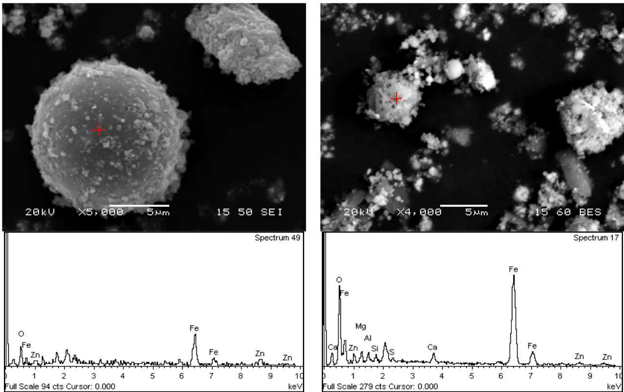
Figure 10: SEM images of the 2 nd step residue (25°C, 2N H 2 SO 4 , 20% pulp density, 10 min). Spherical grain of zinc ferrite (left), magnetite crystal (right)
