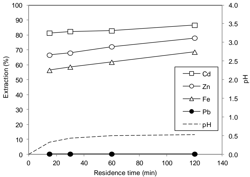
Figure 12: 3 rd step leaching. Extraction (%) of metals vs residence time (95°C, 3N H 2 SO 4 , 20% pulp density).
