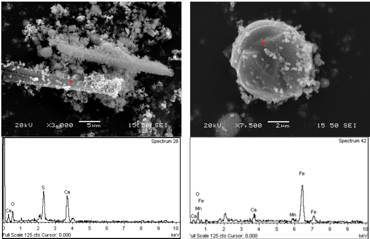
Figure 7: SEM images of washed EAF dust. Plates of calcium sulphate (left) and a spherical particle of magnetite (right).
