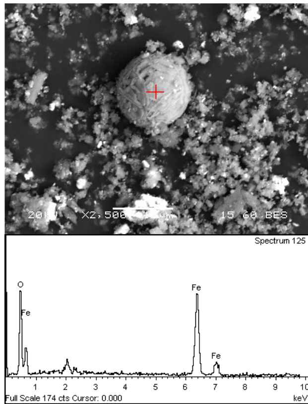
Figure 18: SEM image of the 4 th step leach residue (95°C, 3N H 2 SO 4 , 20% pulp density, 120 min). A corroded by the acid spherical grain of magnetite.
