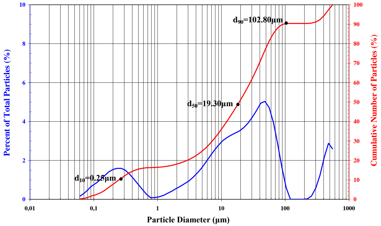
Figure 2: Particle size distribution of the EAF dust processed.
