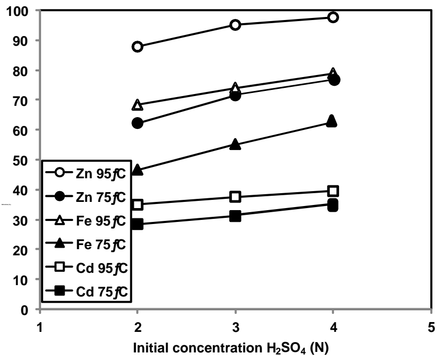
Figure 17: 4 th step leaching. Extraction (%) of metals vs the initial H 2 SO 4 concentration (75 °C and 95°C, 20% pulp density, 120 min).
