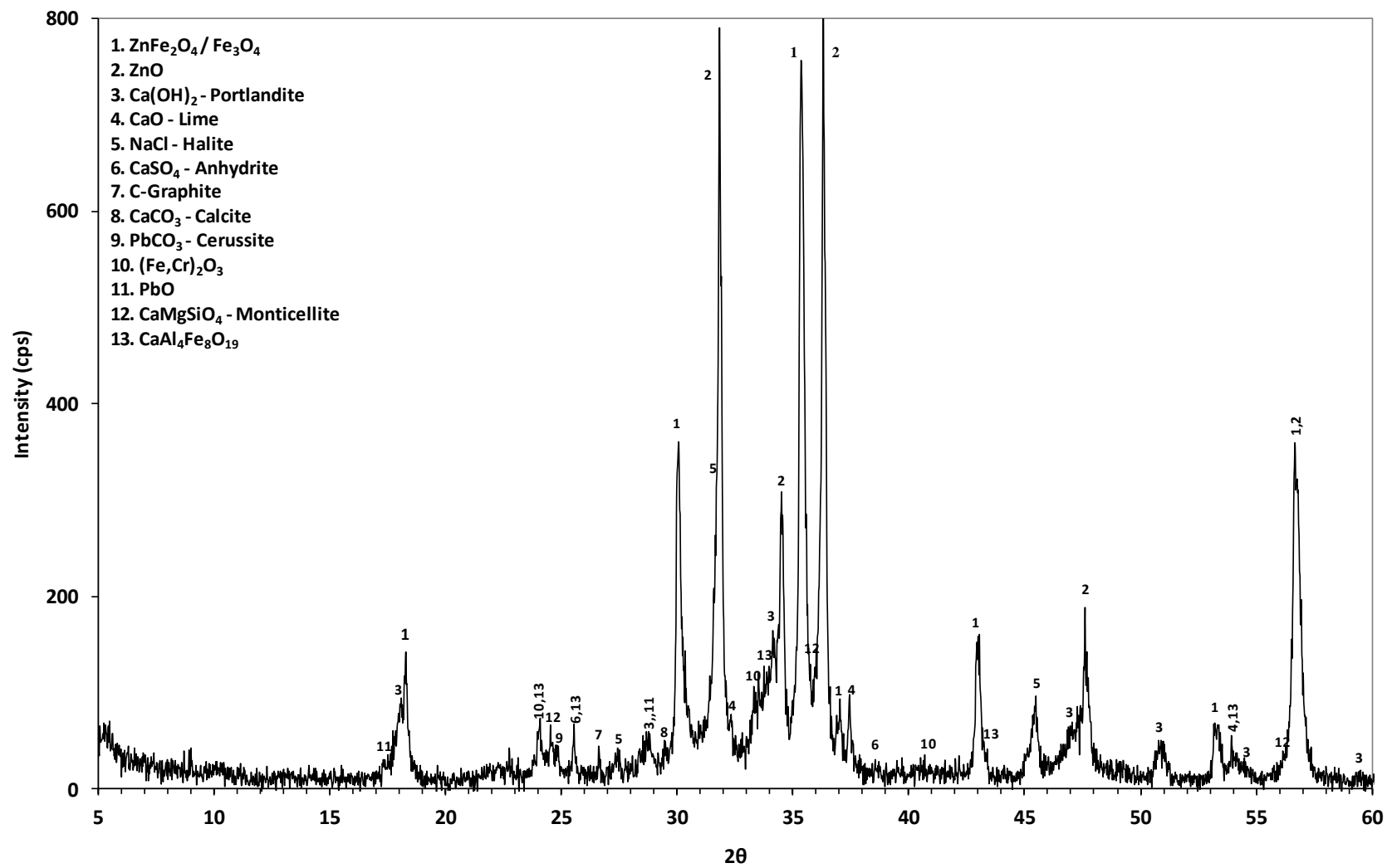
Figure 1: XRD pattern of the EAF dust processed.
