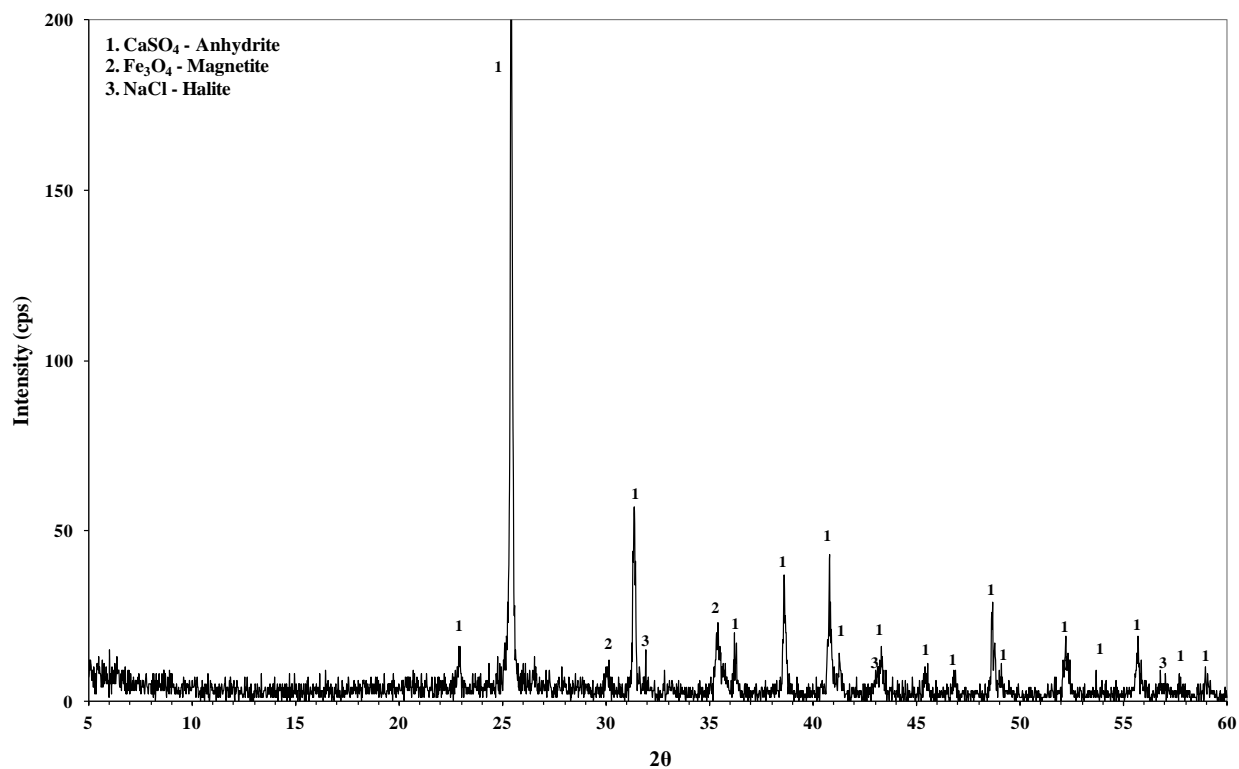
Figure 22: XRD pattern of the residue remaining after leaching with NaCl the lead sulphate leach residue.
