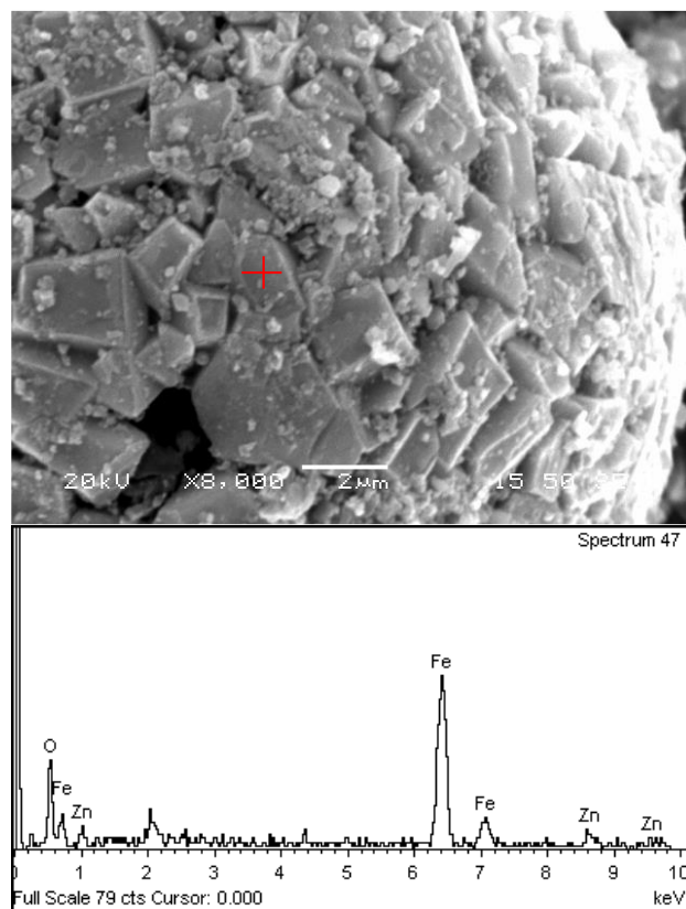
Figure 15: SEM image of the 3 rd step leach residue (95°C, 3N H 2 SO 4 , 20% pulp density, 120 min). A corroded spherical grain of zinc ferrite.
