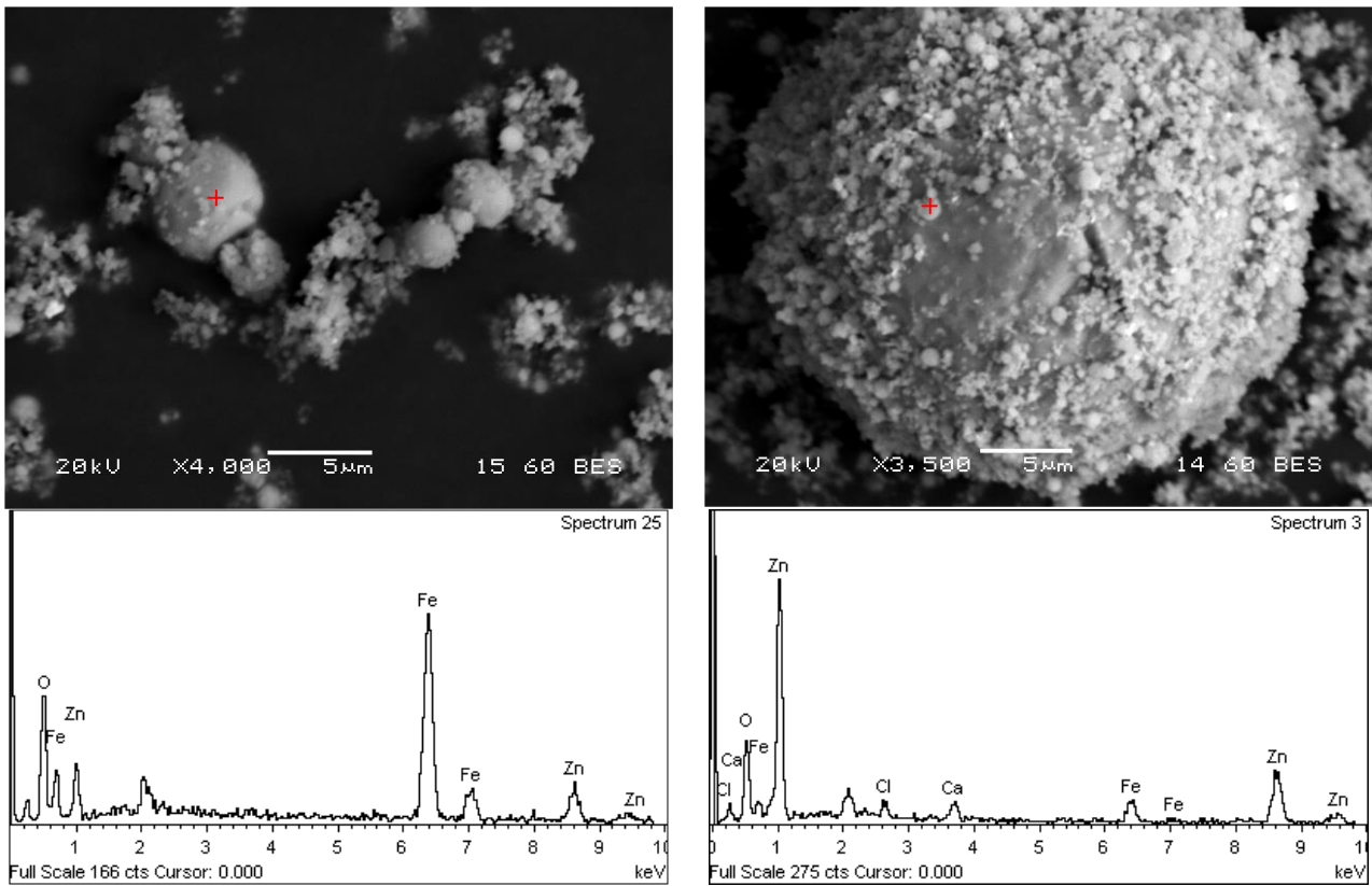
Figure 6: SEM images of washed EAF dust. A sphere of zinc ferrite (left) and fine particles of zinc oxide on the surface of a much bigger spherical particle of zinc ferrite (right).
