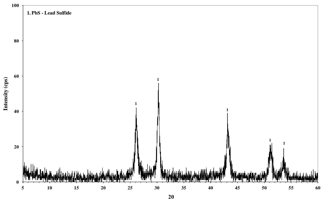
Figure 23: XRD pattern of the lead sulphide, precipitated at 25°C.
