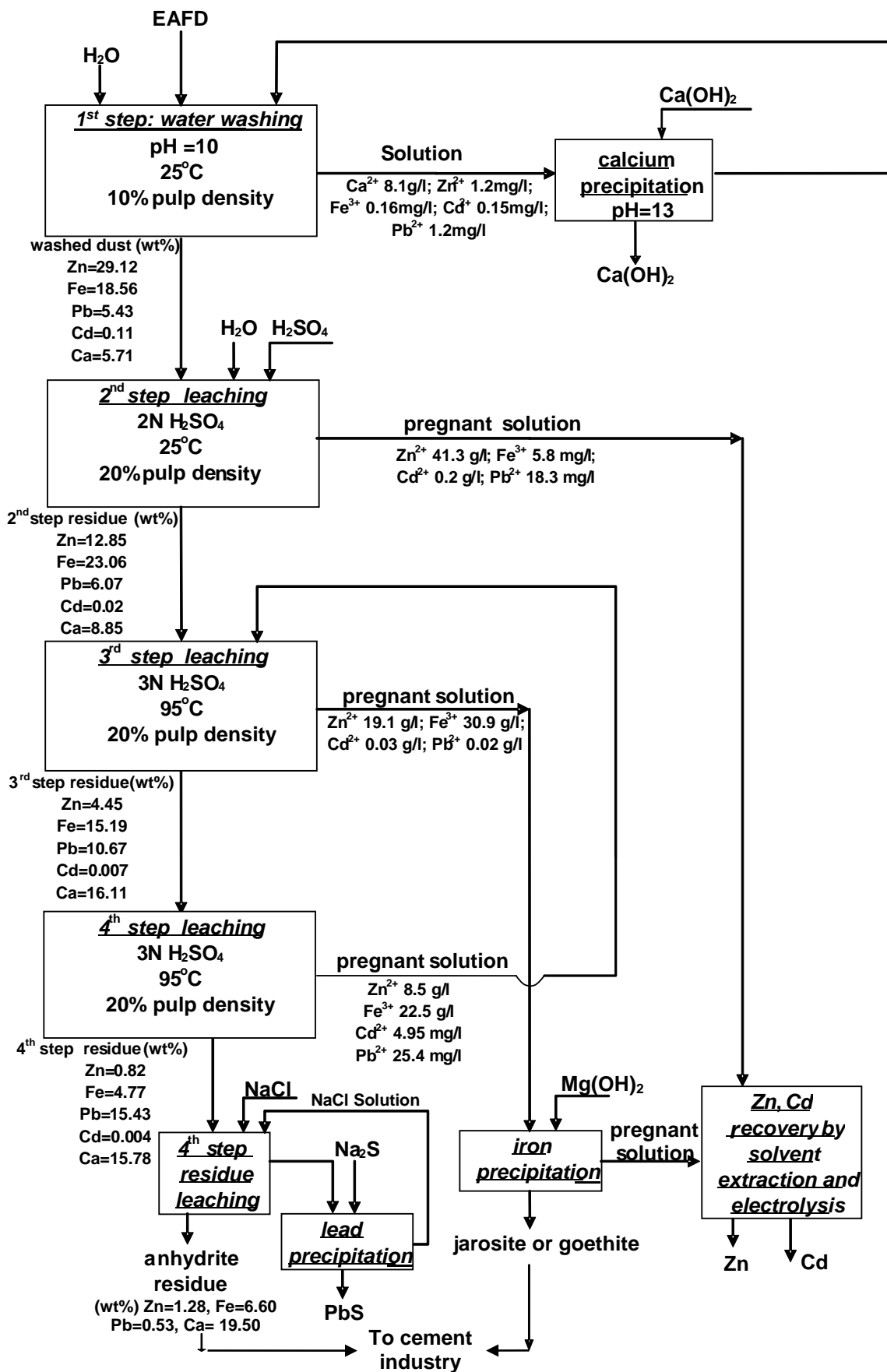
Figure 24: Conceptual flowsheet of the proposed hydrometallurgical method for direct leaching of EAF dust with dilute sulphuric acid at atmospheric pressure.
