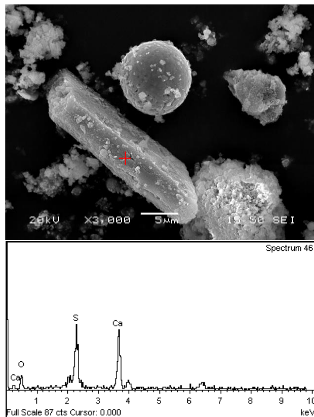
Figure 13: SEM image of the 3 rd step residue (95°C, 3N H 2 SO 4 , 20% pulp density, 120 min). A plate of calcium sulphate.
