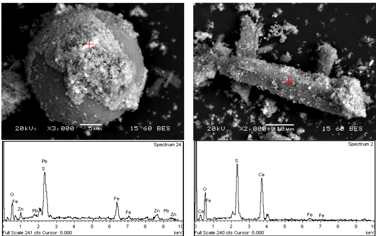
Figure 11: SEM images of the 2 nd step residue (25°C, 2N H 2 SO 4 , 20% pulp density, 10 min). A white crystal of lead sulphate (left), a plate of calcium sulphate (right).
