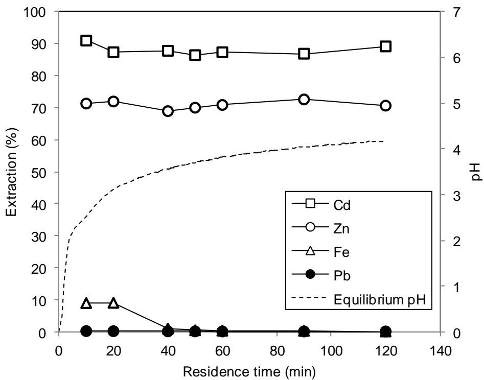
Figure 9: 2 nd step leaching. Extraction (%) of metals vs residence time (25°C, 2N H 2 SO 4 , 20% pulp density).
