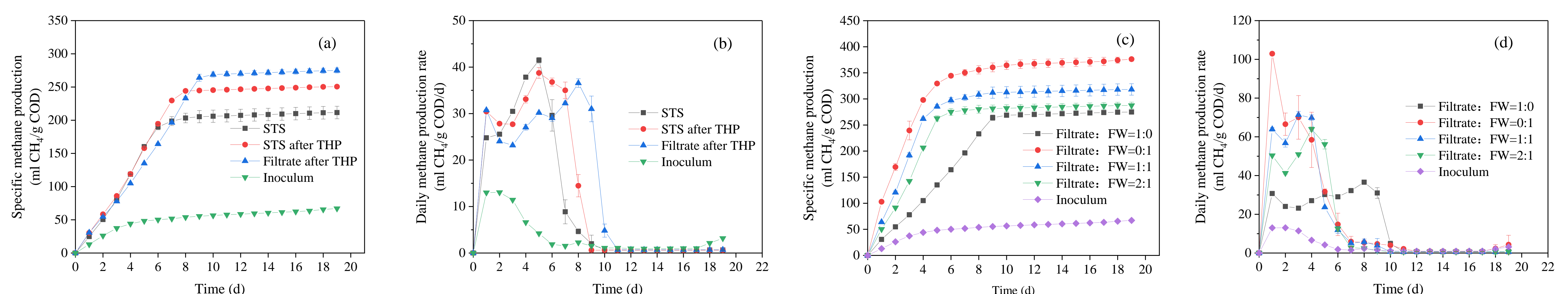
Fig. 1 methane production from septic tank sludge (STS) and food waste (FW) in batch anaerobic digestion (a. and c. accumulative methane production; b. and d. daily methane production)
