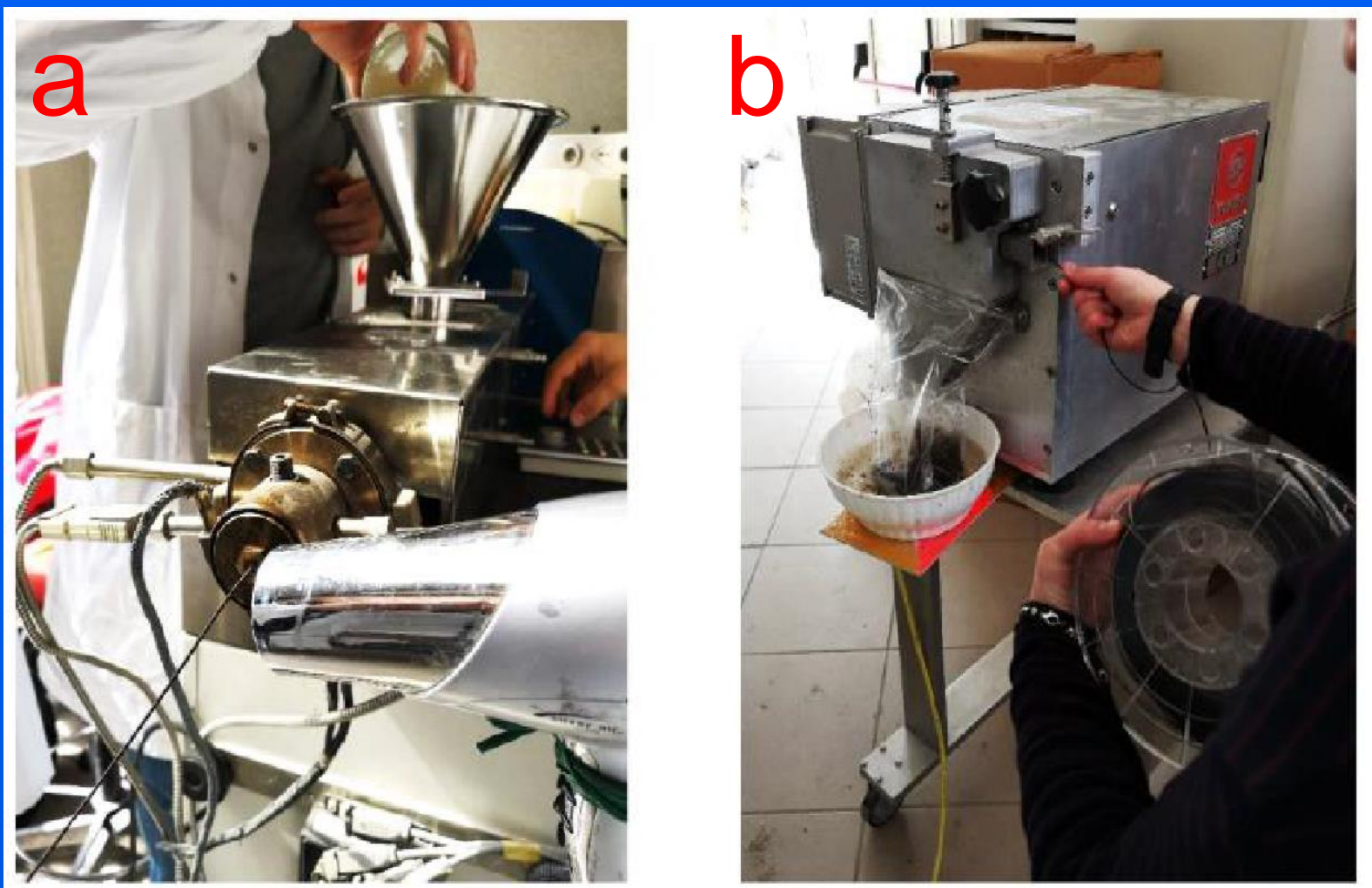
Figure 1: a) extrusion process b) injection molding
